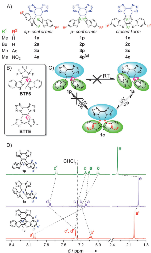
Figure 1. Chemical structures of A) DAEs 1–4 with complete separation of p- and ap-conformers, and corresponding closed forms, and B) reference compounds BTF6 and BTTE with freely rotatable aryl groups. C) The conversion relationship of 1a, 1p, and 1c with a hindered aryl group. D) Comparison of 1 H NMR spectra of 1p, 1a, and 1c in CDCl 3 . [a] 4p was not obtained owing to the direct nitration of 1a, resulting in only 4a.
